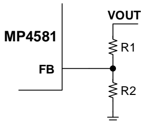
Figure 2: Feedback Network
