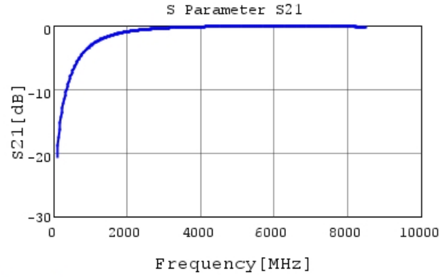
GRM1555C1H1R5CA01 S21 DCOV, 25degC
