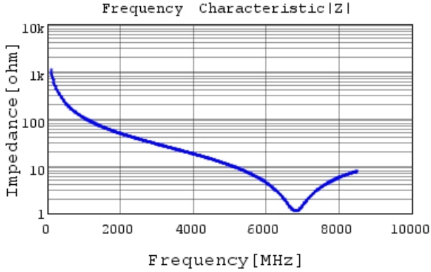
GRM1555C1H1R5CA01 |Z| DC0V, 25degC
