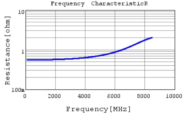
GRM1555C1H1R5CA01 R DC0V, 25degC
