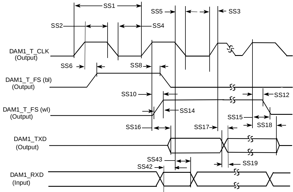
Figure 80. SSI Transmitter with Internal Clock Timing Diagram
