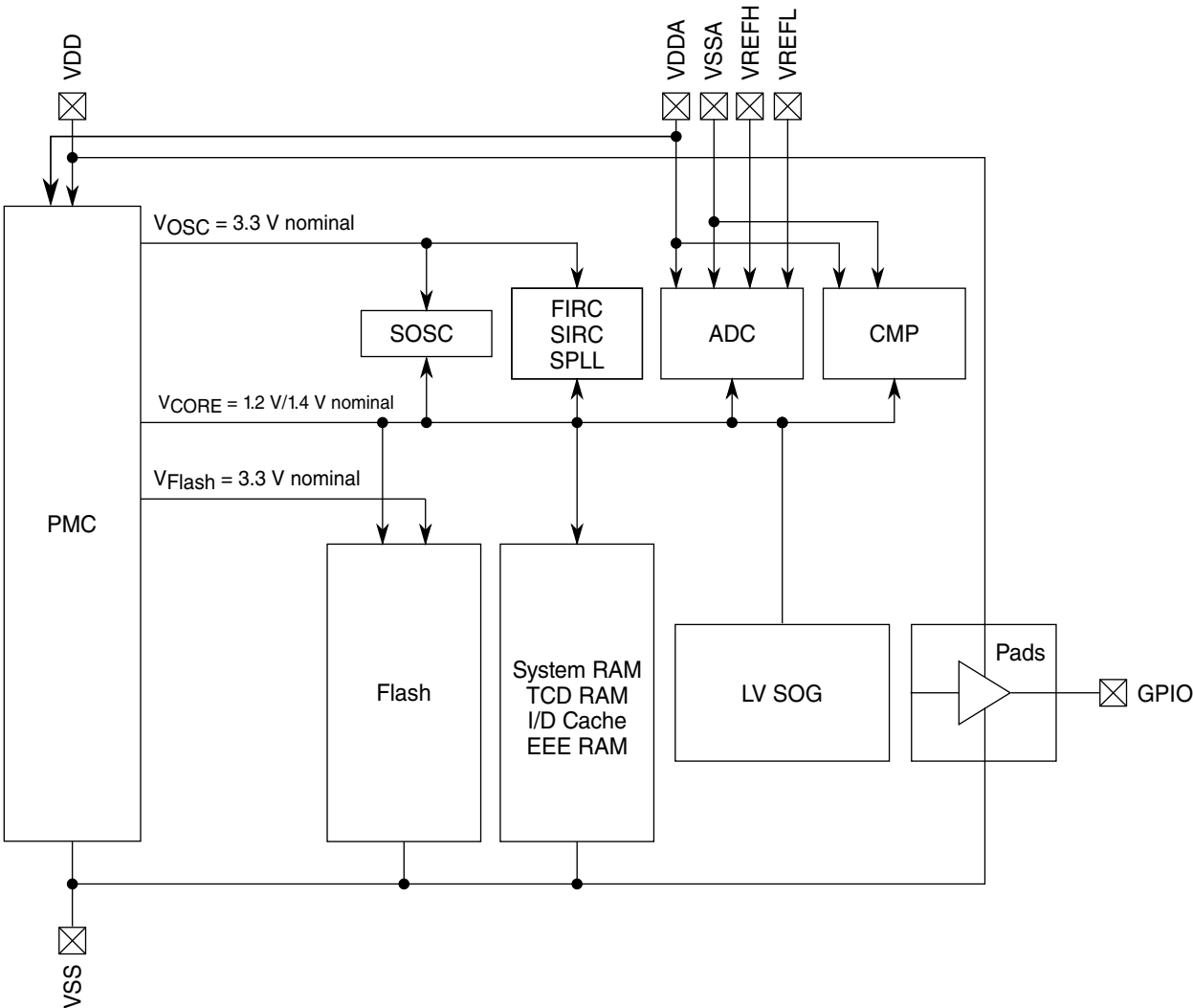
Figure 6. Power diagram
