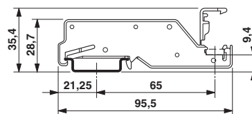
Dimensioned drawing
