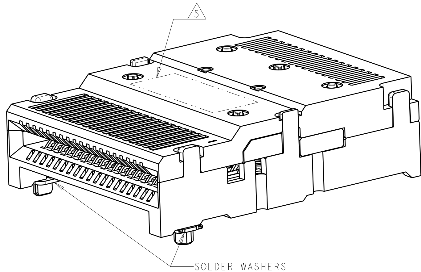
2318579-2 WITH SOLDER WASHERS SCALE 6:1
