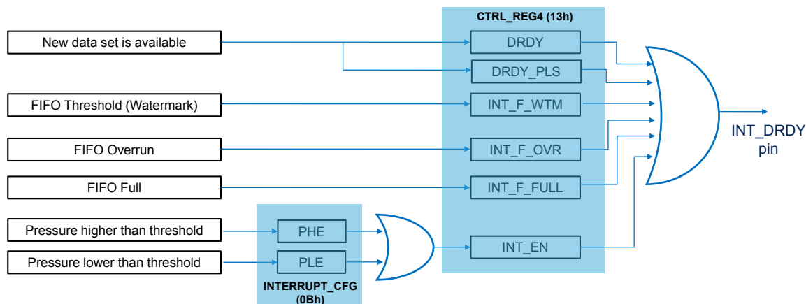
Figure 17. Interrupt events on INT_DRDY pin
