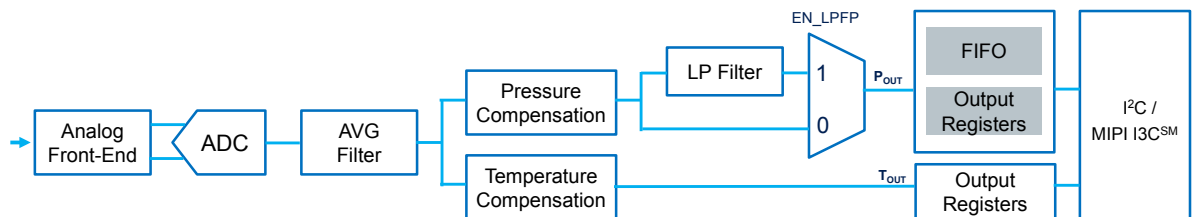
Figure 2. Digital logic
