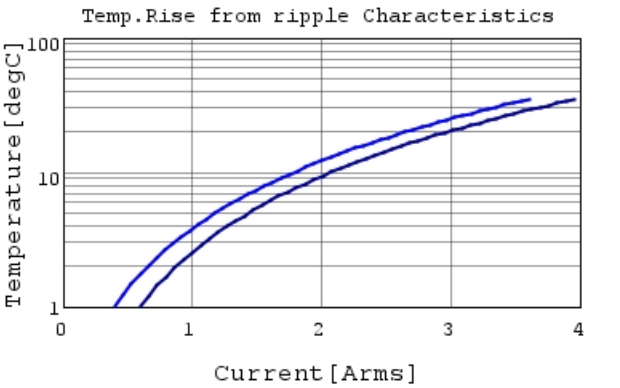
GRM188R61C225KE15 Temp.rise — 500kHz —
