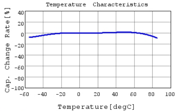
GRM188R61C225KE15 C-Temp. capchange, DC0.0V,
