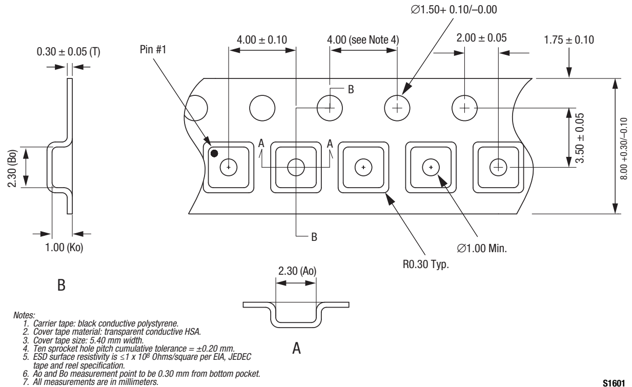
Figure 11. CLA4605-085LF Tape and Reel Dimensions
