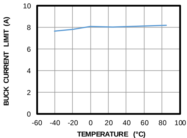
Buck Current Limit vs. Temperature
