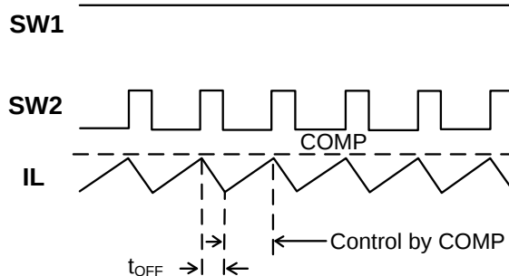
Figure 5: Boost Waveform
