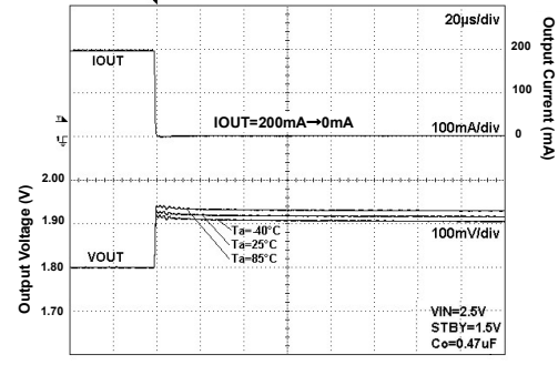
Fig 19. Load Response
